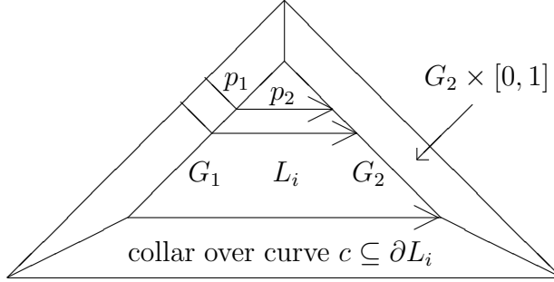
FIGURE 1. Schematic for collapsing map
