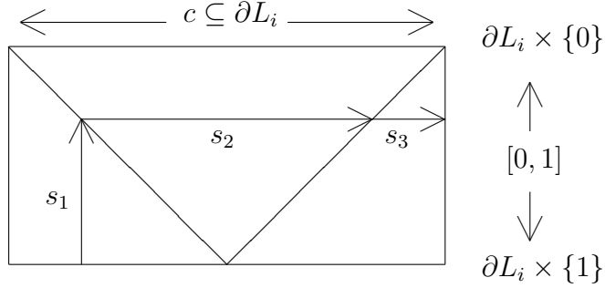
FIGURE 2. Defining g_{i+1} on collar portion over curve c \subseteq \partial L_i
